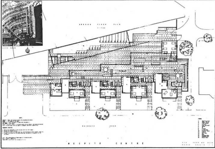
Ground-floor plan.
